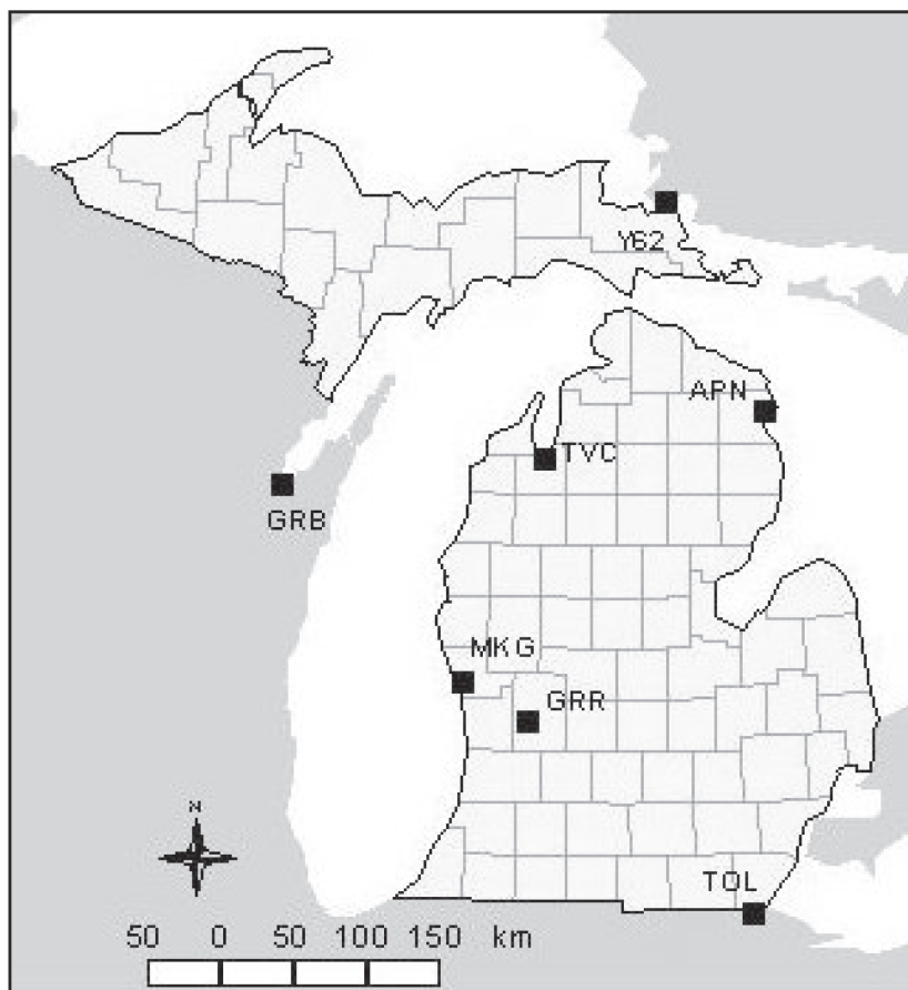
Fig. 1. National Weather Service (NWS) stations used in historical trend analysis: Sault Ste Marie, Mich. (Y62); Alpena, Mich. (APN); Traverse City, Mich. (TVC); Green Bay, Wis. (GRB); Muskegon, Mich. (MKG); Grand Rapids, Mich. (GRR); Toledo, Ohio (TOL).
